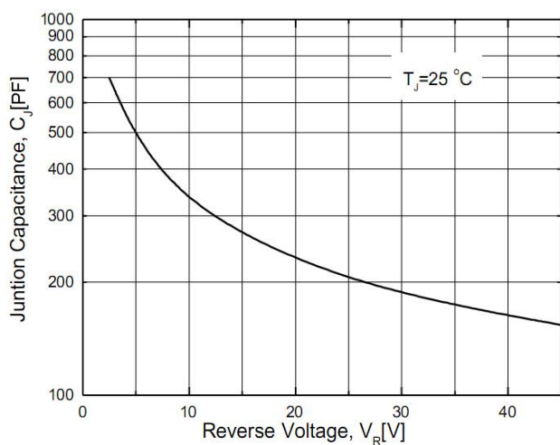
Figure 3. Junction Capacitance
