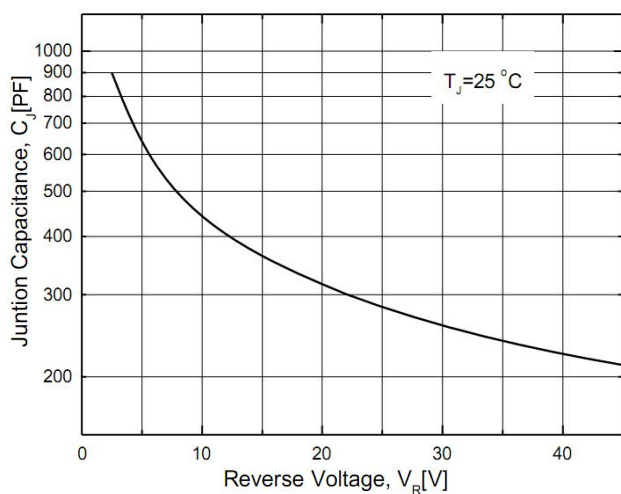
Figure 3. Junction Capacitance
