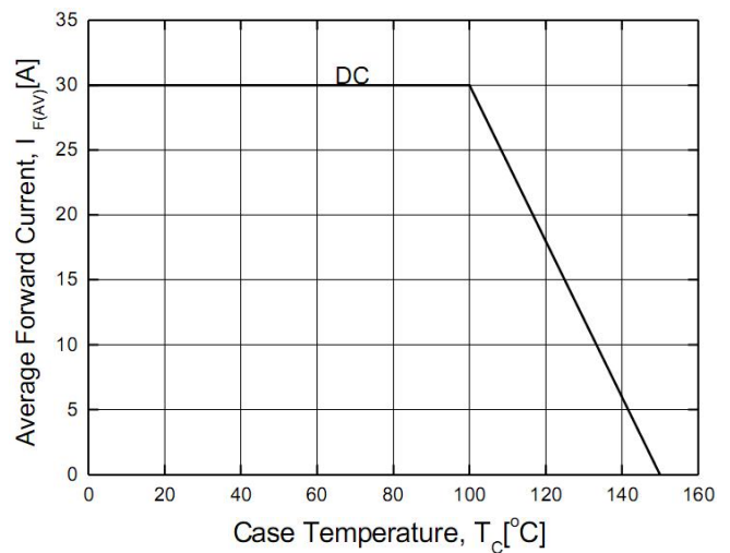
Figure 4. Power Derating
