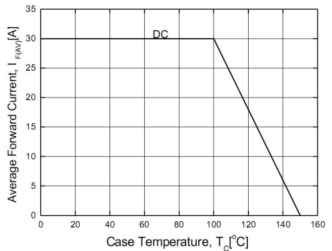
Figure 4. Power Derating
